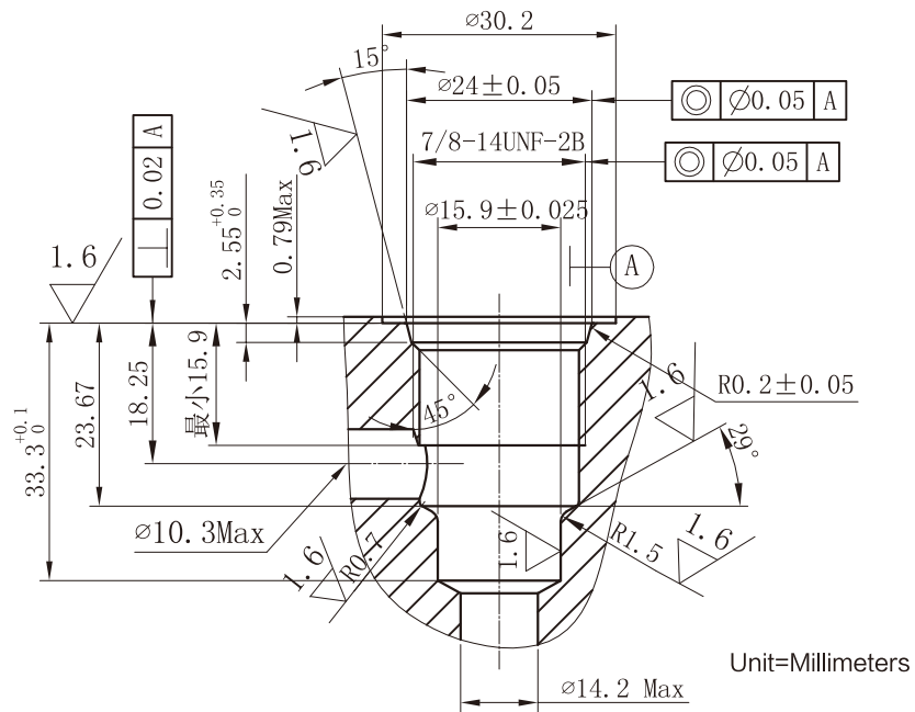
CAVITY 插孔: 10-2
